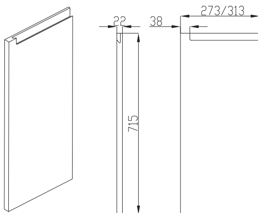
Base Door LH 313mm wide
