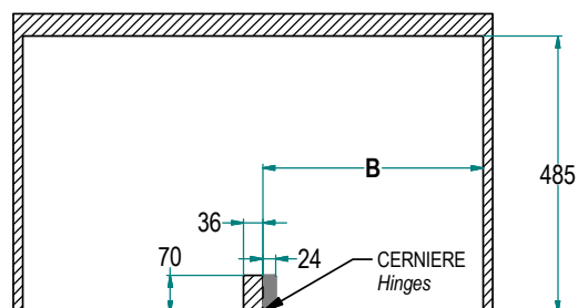
Dimensioni mobile Cabinet dimension
