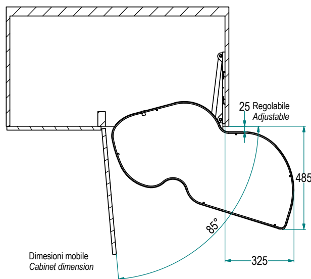
Ingombro vassoio estratto Extracted tray overall dimensions
