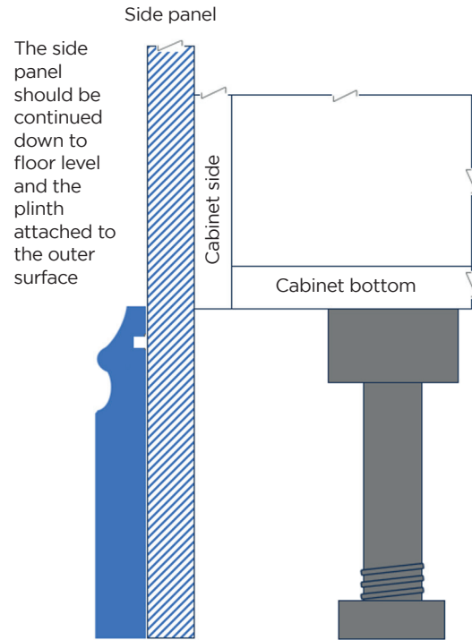
Side view showing plinth wrapping around end panels
