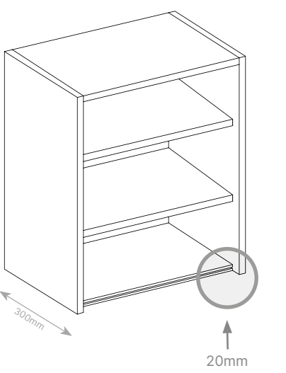
Base panel set back & groove routed for profile
