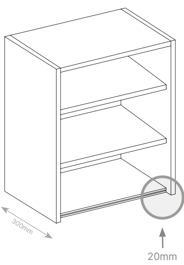
Base panel set back & groove routed for profile
