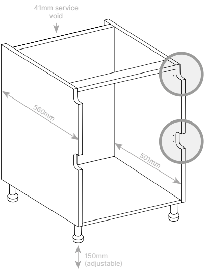
Top and mid sections pre-routed Pre-drilled holes for quick fix brackets
